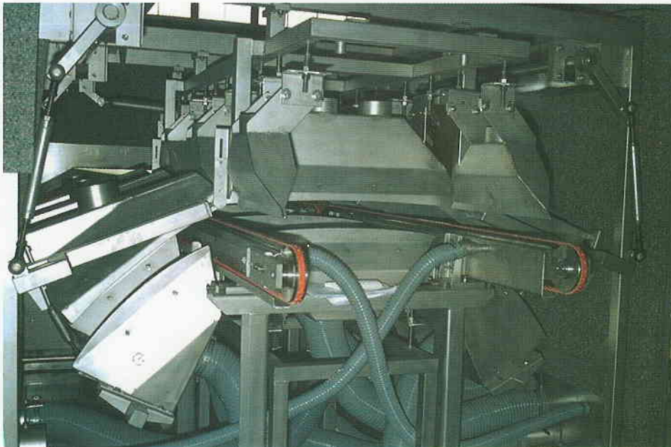
Drying Section with adjustable Air Knives (smile adjusting)
